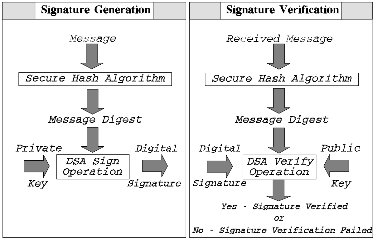
Figure 1: Using the SHA with the DSA
